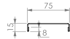
REINFORCING CHANNEL II DETAIL
