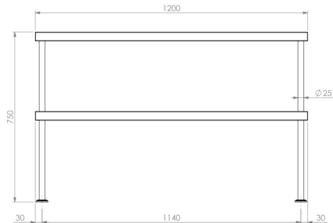
FRONT ELEVATION
