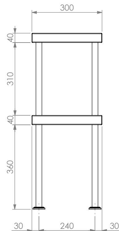
SIDE ELEVATION
