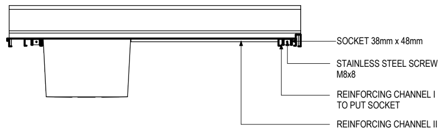
A-SECTION VIEW SCALE 1:15mm
