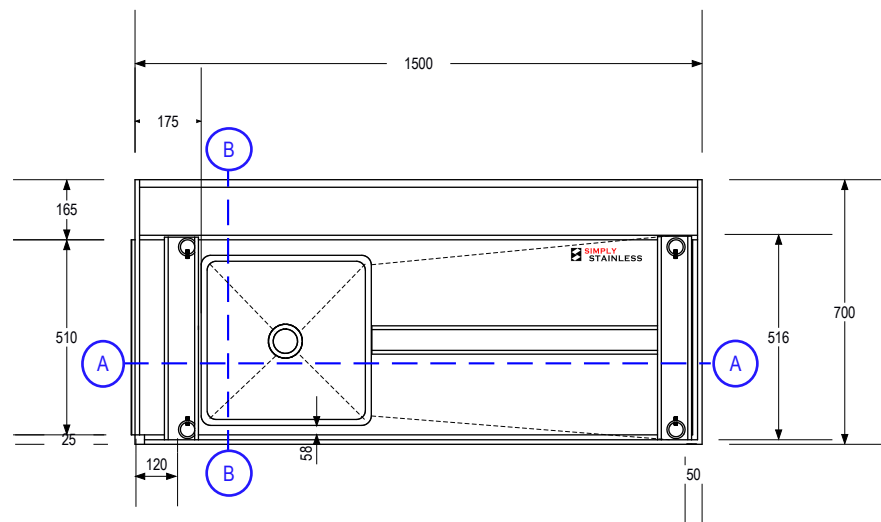
BOTTOM-PLAN VIEW (TOP ONLY)
