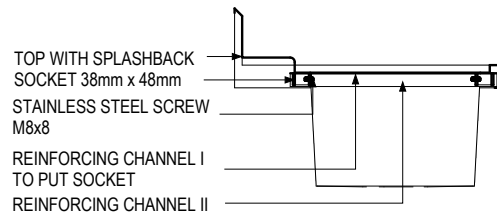
B-SECTION VIEW SCALE 1:15mm
