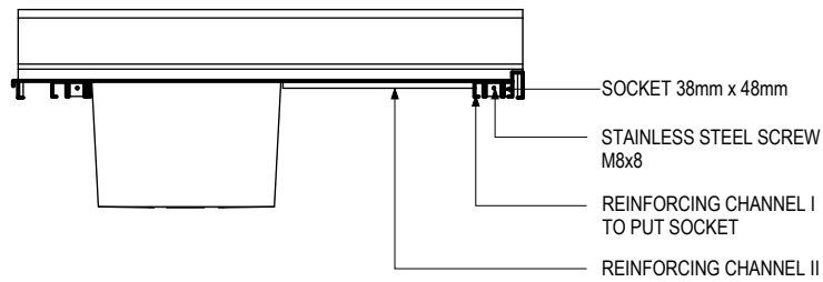
A-SECTION VIEW SCALE 1:15mm
