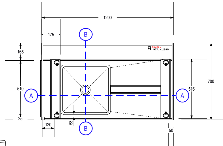
BOTTOM-PLAN VIEW (TOP ONLY)
