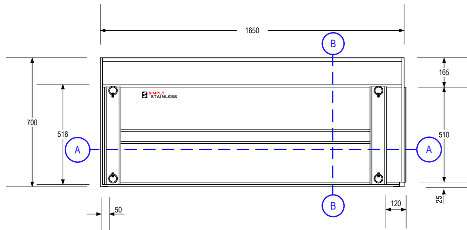
BOTTOM-PLAN VIEW (TOP ONLY)
