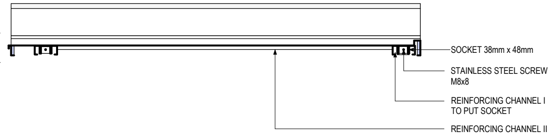
A-SECTION VIEW SCALE 1:15mm
