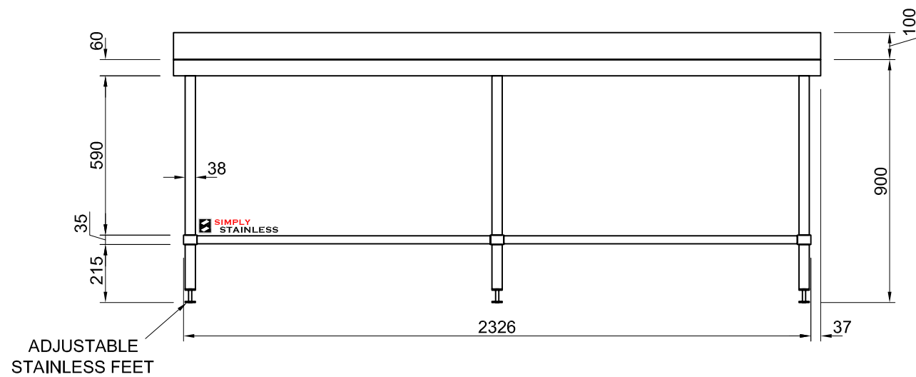
FRONT ELEVATION
