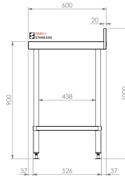
SIDE ELEVATION
