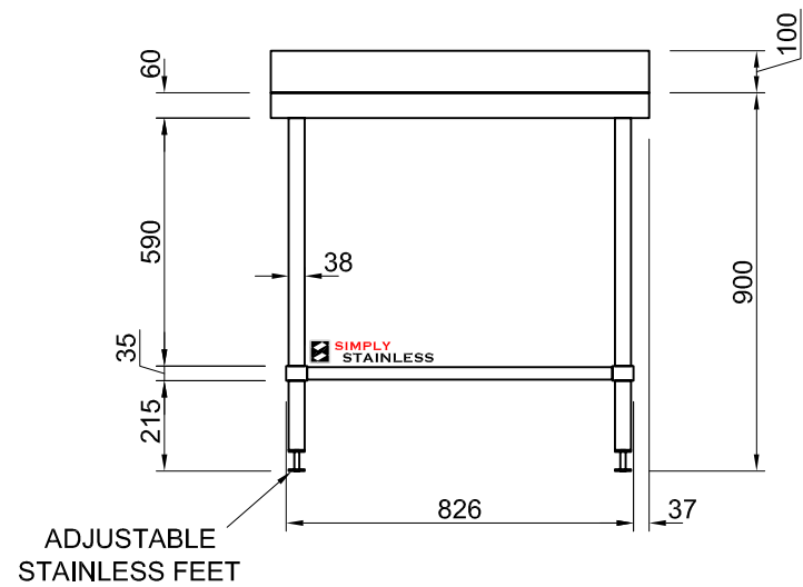
FRONT ELEVATION
