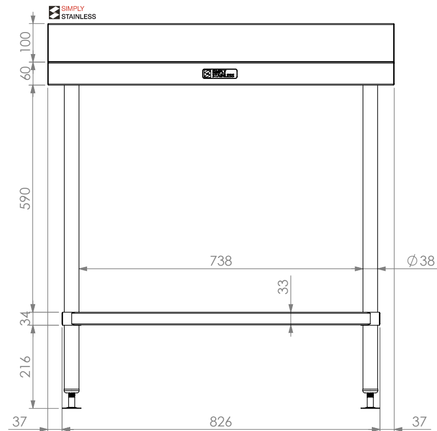
FRONT ELEVATION
