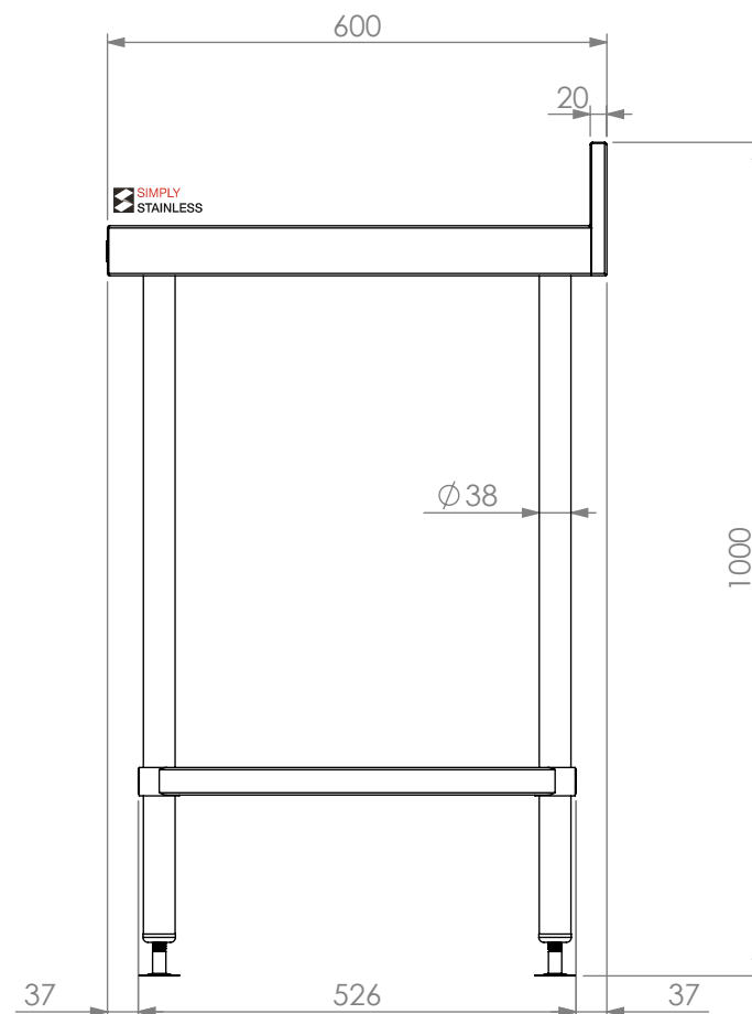
SIDE ELEVATION
