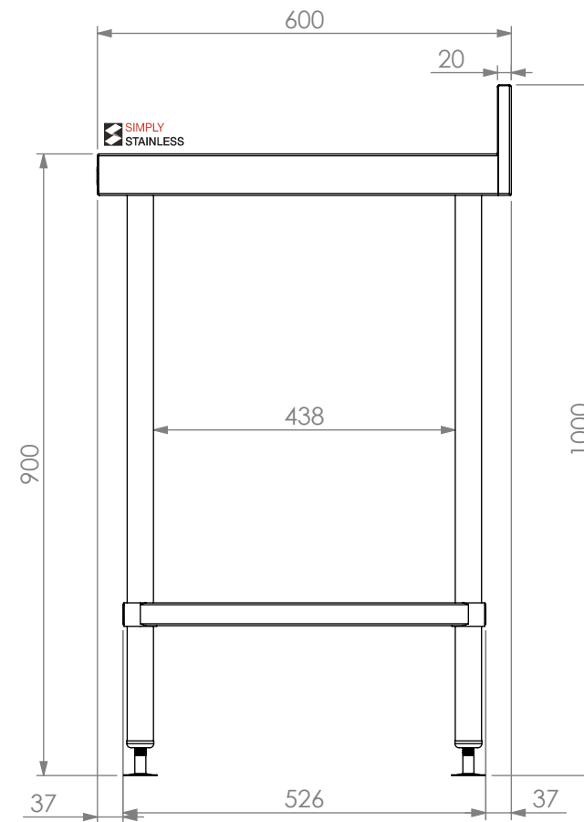
SIDE ELEVATION
