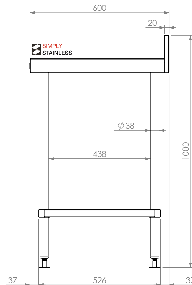
SIDE ELEVATION
