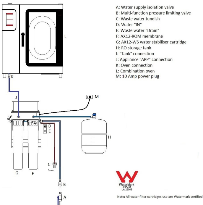
QuadRO H200 Installation Diagram
