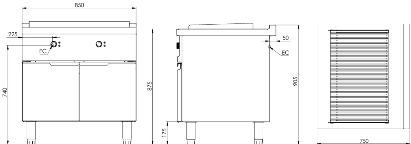
EG 6CC 800 CBM
