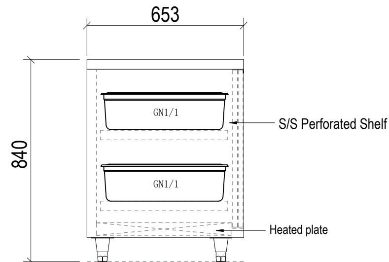
SIDE VIEW
