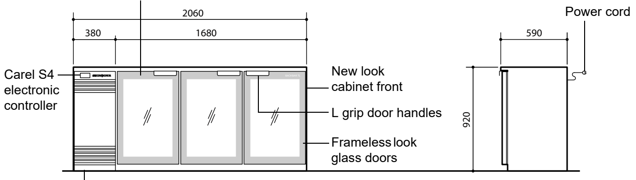
Side mounted integral refrigeration unit
