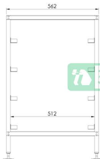
Front
